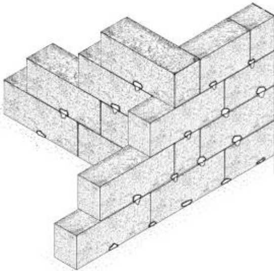
SCARF BETWEEN WALL AND PARTITION
