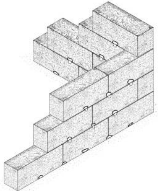
CORNER SCARF
